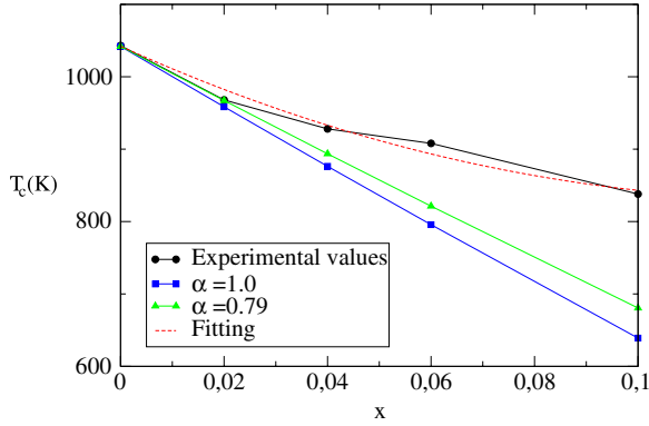
Figure 1. Critical temperature as a function of the Ru concentration. Experimental points are represented by circles. Squares (triangles) represent constant AF interactions, J_{AF} , with J_{AF}/J = 1.0 (0.79), where J is the strength of the ferromagnetic interaction between Fe atoms. The dashed line represents results from a least-square fitting taking into account that J_{AF} varies with x in the form J_{AF} = 0.54 - 5.4 x .
