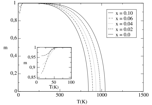
Figure 2. Magnetization versus temperature for five different x values. The inset shows details of the magnetization behavior at low temperatures. The legends are the same for the two graphs; the outermost curve corresponds to x = 0 while the innermost one is for x = 0.10 .
